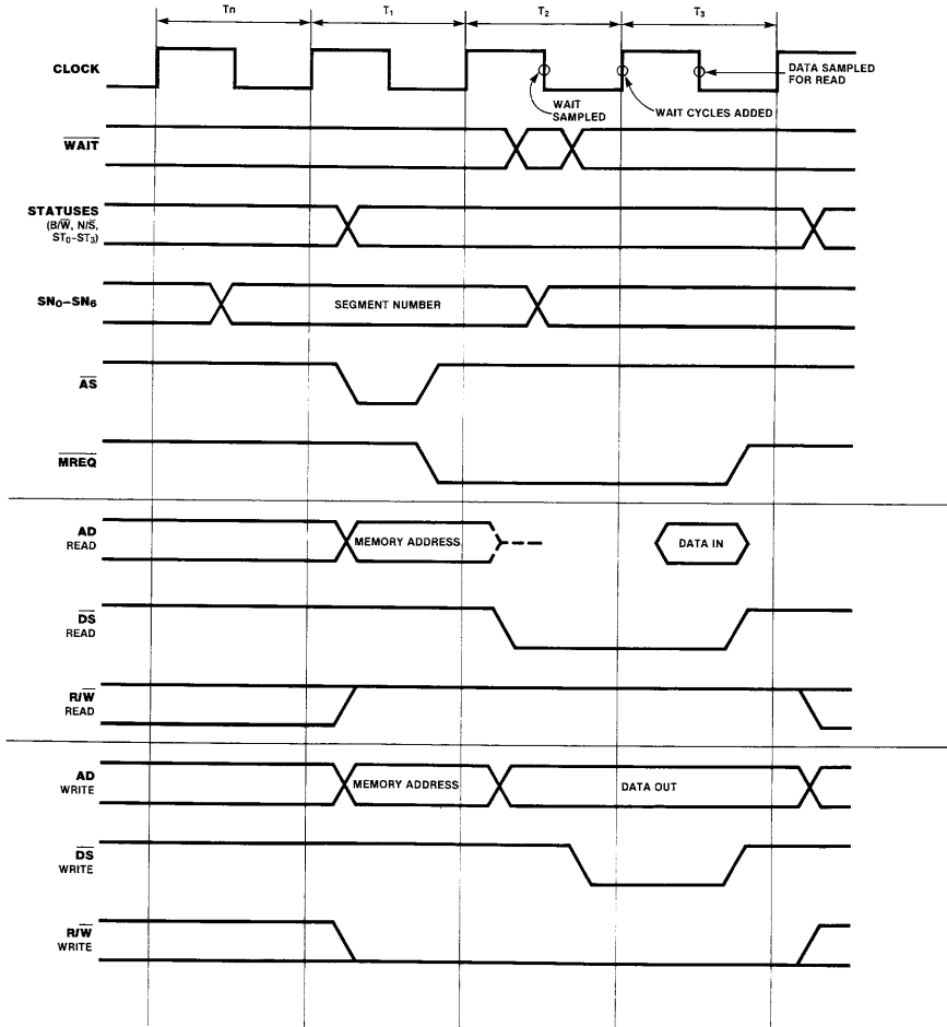
Figure 9-3. Memory Read and Write Transaction
