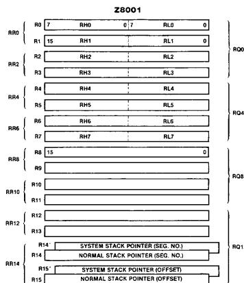
Figure 2-5a. Z8001 Segmented General-Purpose Registers (Register Address Space)
