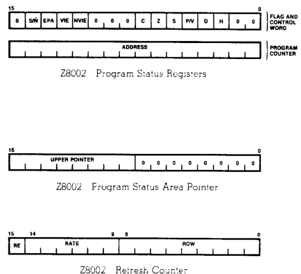
Figure 4-2. Program Status Registers
