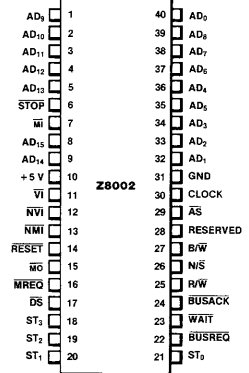
Z8002 Pin Assignments
