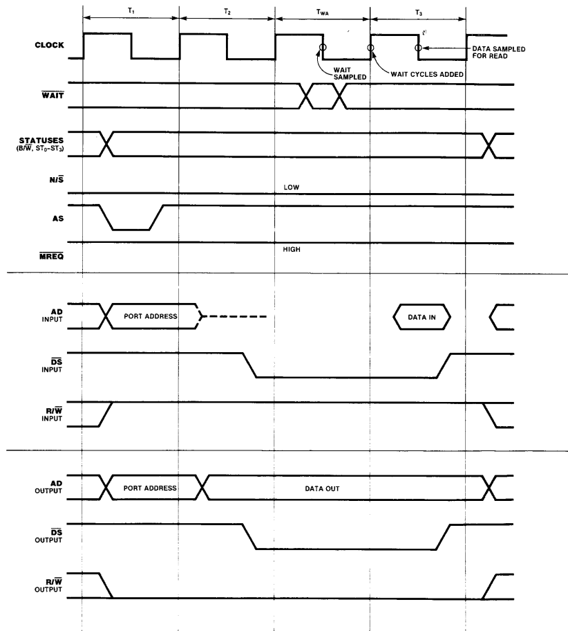
Figure 9-5. Input/Output Transaction
