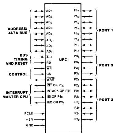
Figure 1. Pin Functions
