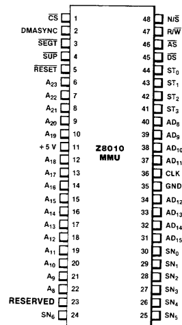
Figure 2. Pin Assignments
