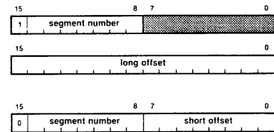
Figure 5-2. Segmented Memory Address Within Instruction.
