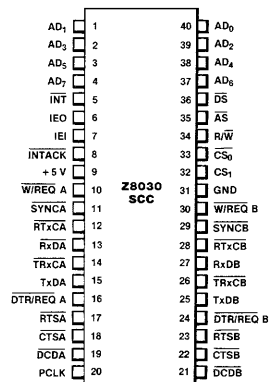
Figure 2. Pin Assignments
