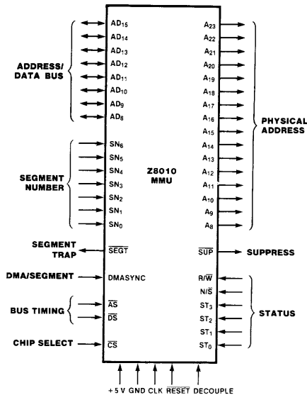
Figure 1. Pin Functions
