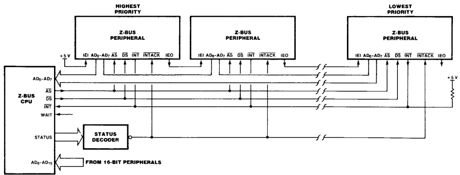
Figure 2. Interrupt Connections
