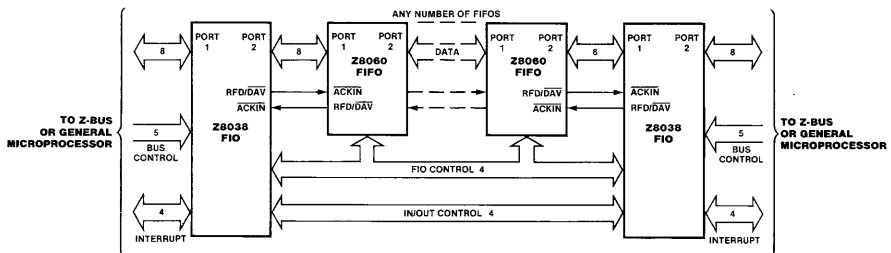
Figure 2. Using FIFOs to Extend FIOs
