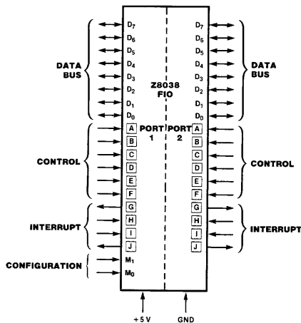
Figure 1. Pin Functions
