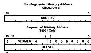
Figure 3-3. Segmented and Non-Segmented Address Formats
