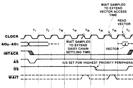
Figure 3. Interrupt Acknowledge Timing
