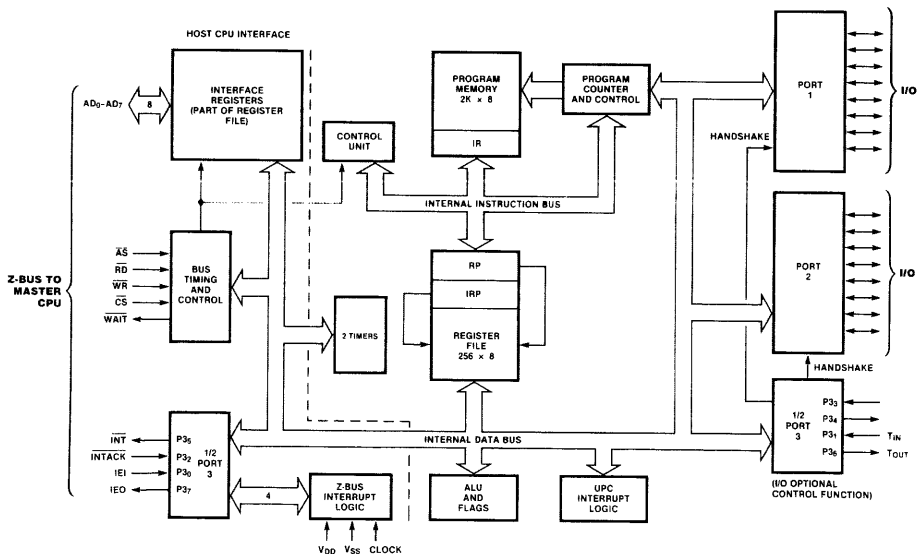
Figure 3. Z-UPC Functional Block Diagram
