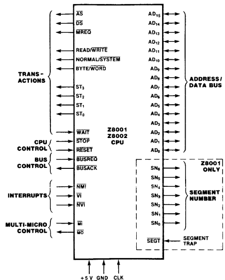
Figure 9-1. Pin Functions
