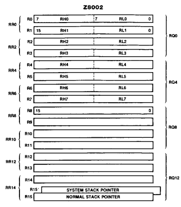
Figure 2-5b. Z8002 Nonsegmented General-Purpose Registers (Registers Address Space)
