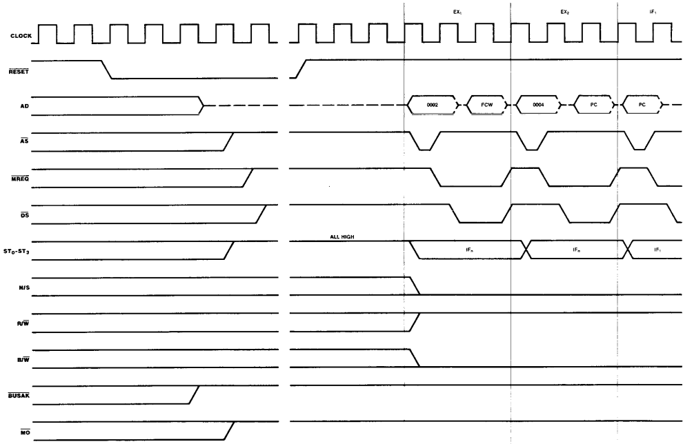
Figure 9-11. Reset Timing
